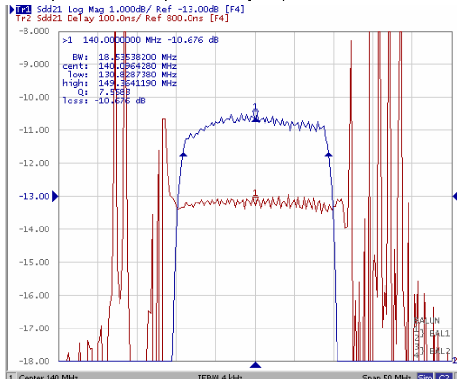
Fig2. Horizontal: 5MHz/Div Vertical: 1dB/Div
